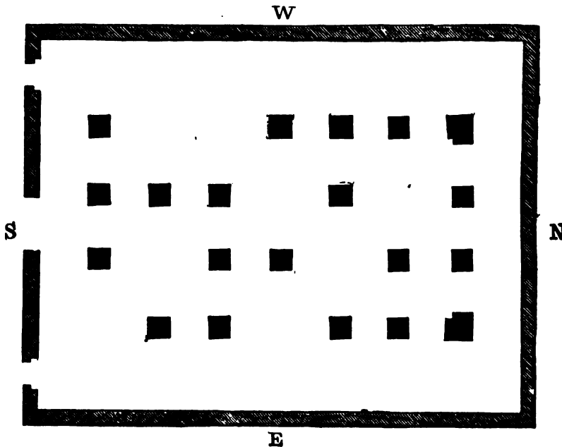
PLAN OF SYNAGOGUE AT 'TELL HUM.'
